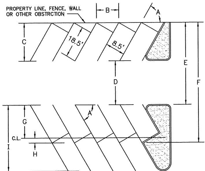
TYPICAL ABUTTING PARKING BAY WITH OVER-LAPPING STALLS
